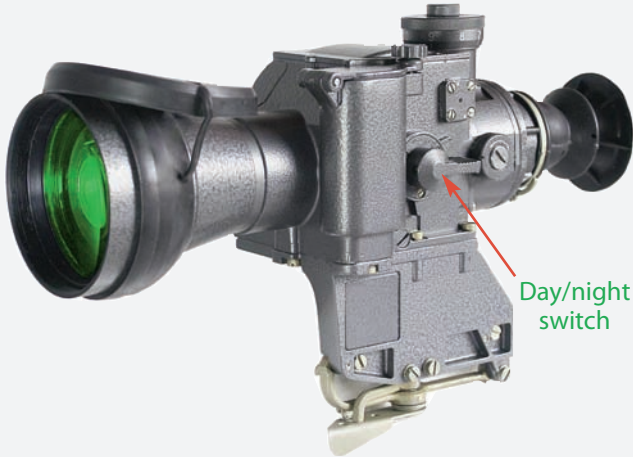
NVS 10MG with side mount
