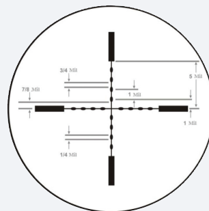
Mil-Dot Reticle Pattern
